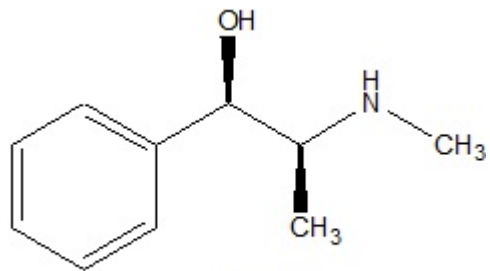
Ephedrine
