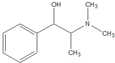
Methylephedrine
